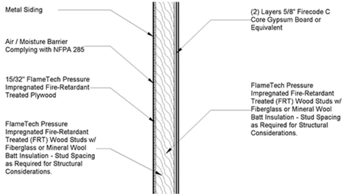
② FRCT/FRWT 120-01 - Section (Typ.) 3/4" = 1'-0"
