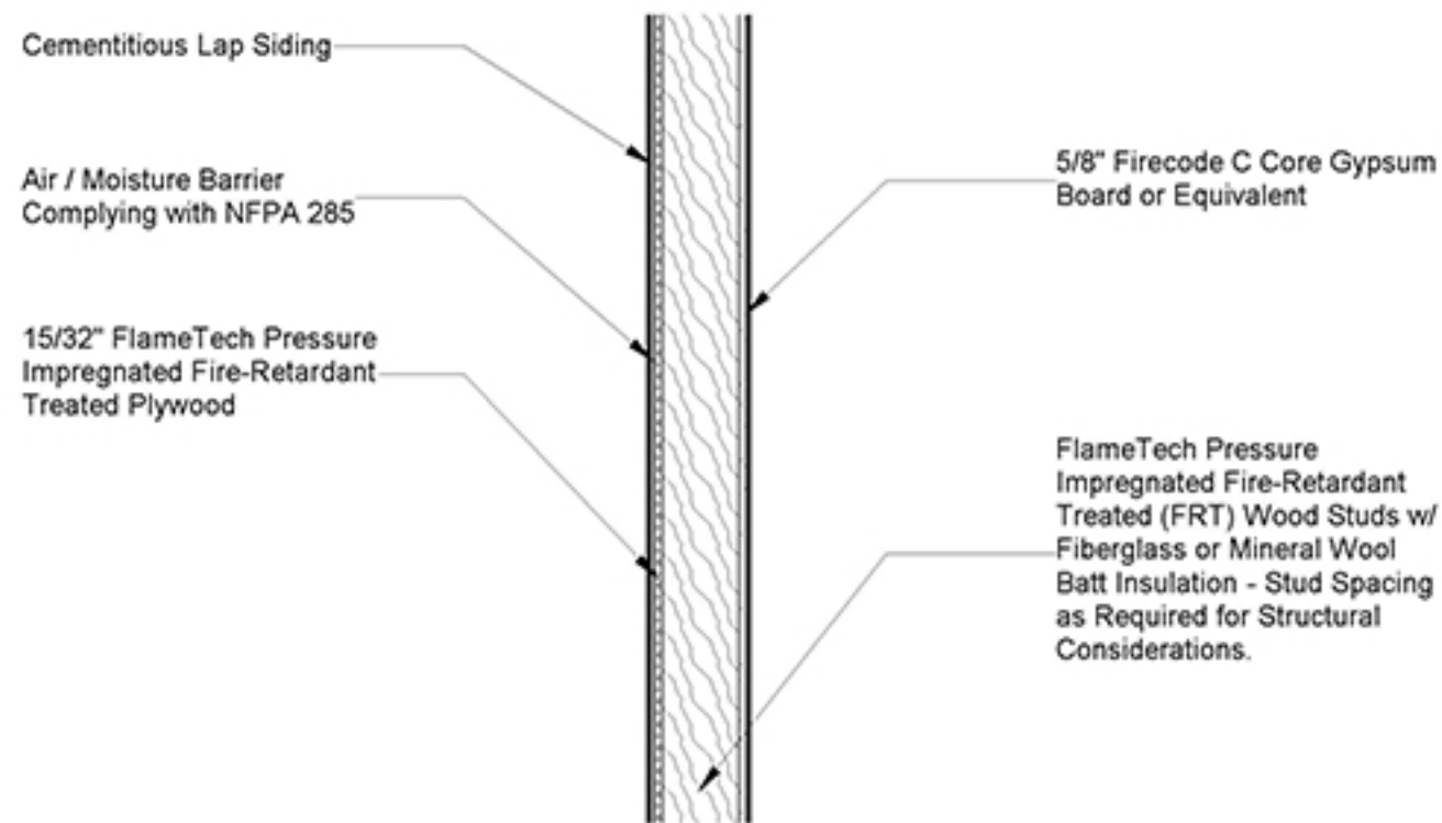
2 FRCT/FRWT 60-01 - Section (Typ.) 3/4" = 1'-0"
