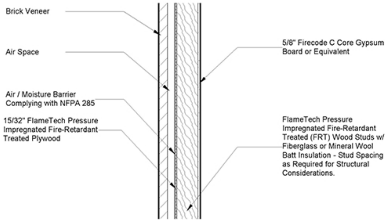
② FRCT/FRWT 60-02 - Section (Typ.) 3/4" = 1'-0"
